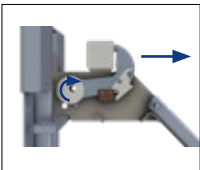
Advanced cam design rotates hook away from RIG first to release pressure from "RIG wedge."
